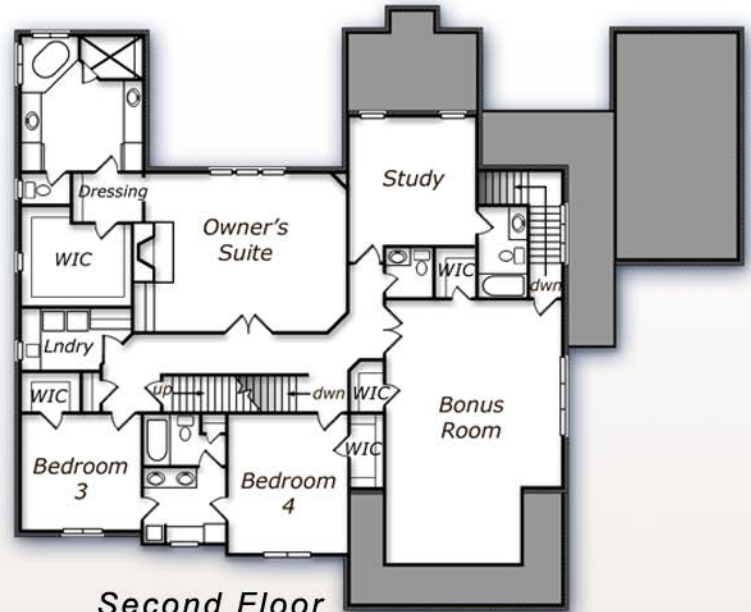
Second Floor
